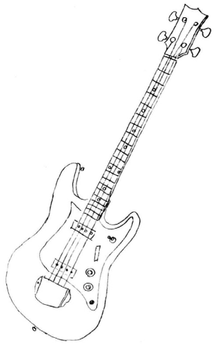
Bass Guitar
